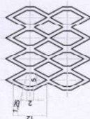
PLATED STEEL INNER MESH DETAIL SCALE 3:1
