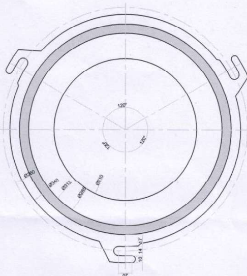
DETAIL OF TOP FLANGE (ALLUMINIUM FLANGE 3-LUG)
