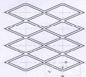
PLATED STEEL OUTER MESH DETAIL SCALE 2:1
